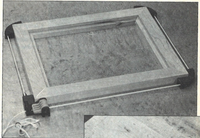
The Wolfcraft Cord Clamp (above and to the right) does not apply a lot of pressure, but this makes it possible to adjust for square and to rapidly slide the clamp off and onto another frame.
