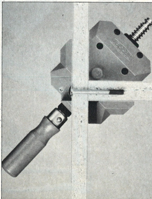
The pivoting jaw of the Bessey WS-3 permits clamping of pieces that are different thicknesses.
