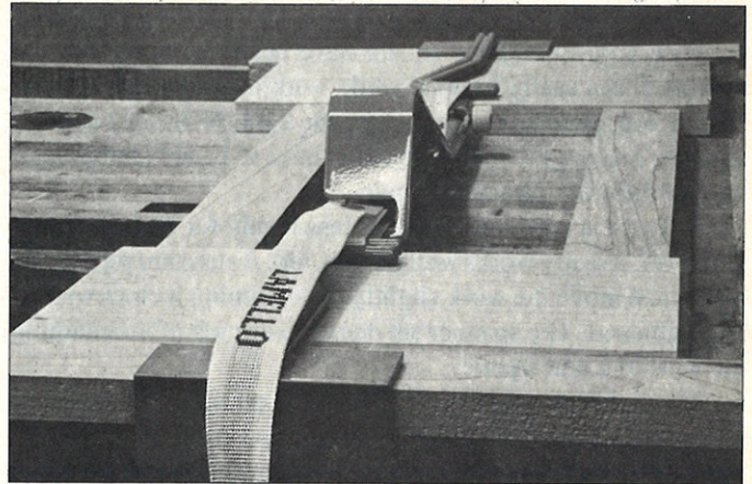
Clamping flat assemblies is quick and easy with the Lamello Spanner Set.
