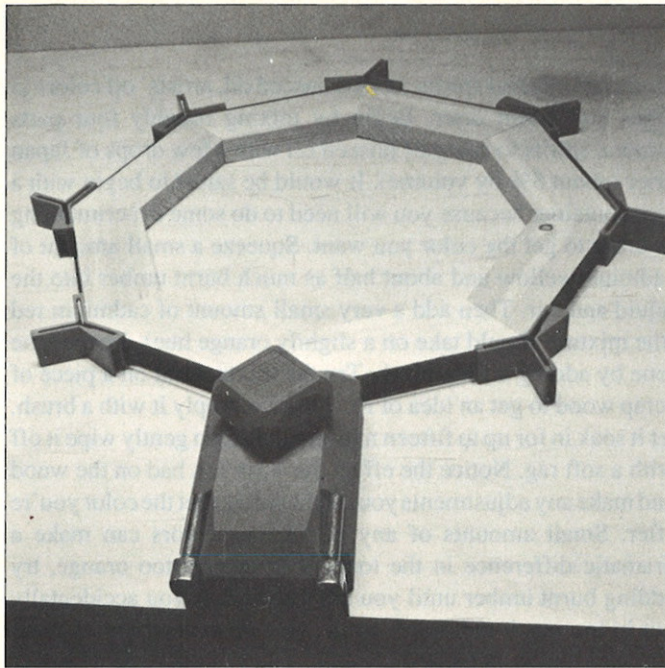
The Bessey Poly-Angle Strap Clamp's corner pieces are shaped in such a way that, depending on how they are fitted on the strap, they will clamp four-, six- or eight-sided objects. The base itself can also be clamped to the work surface.
