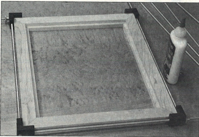
The threaded rods allow the Pony Four Corner Framing Clamp to maintain its shape for mass-producing frames that are all the same size.
