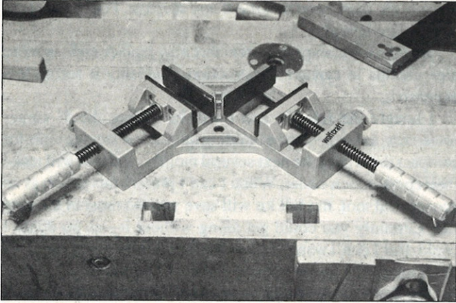
The Wolfcraft Miter Vise features quick-action jaws for rapid assembly of mitered joints.
