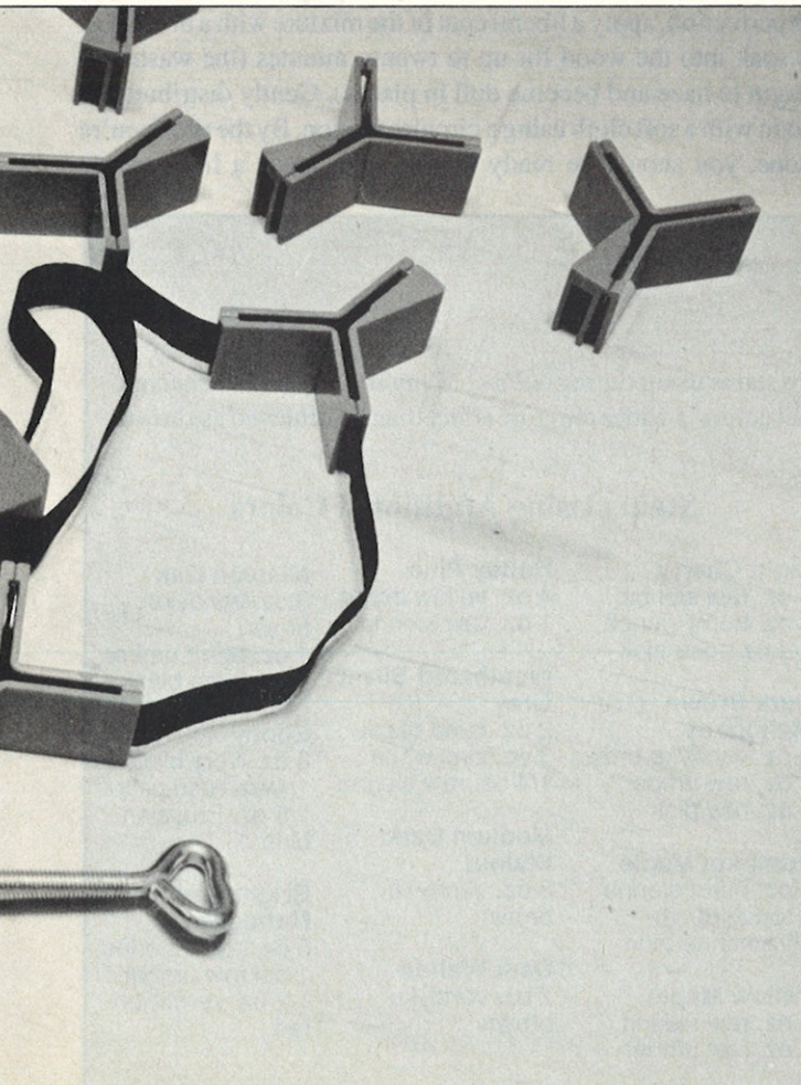
The Bessey Poly-Angle Strap Clamp's corner pieces are shaped in such a way that, depending on how they are fitted on the strap, they will clamp four-, six- or eight-sided objects. The base itself can also be clamped to the work surface.
