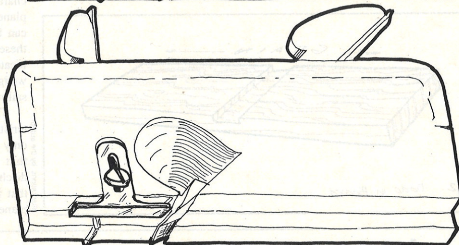
Side-mounted Depth stop
