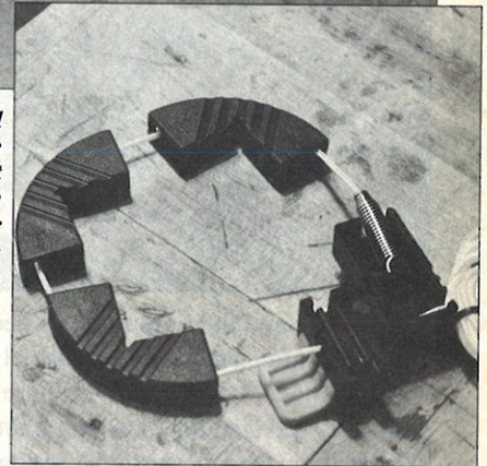
The Wolfcraft Cord Clamp (above and to the right) does not apply a lot of pressure, but this makes it possible to adjust for square and to rapidly slide the clamp off and onto another frame.
