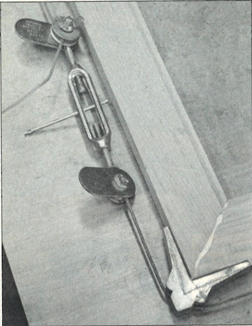
The Jiffy Clamp's wire cable is drawn tight with a turnbuckle.
